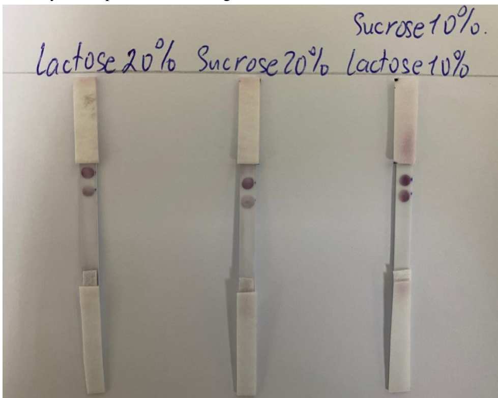
Figure 4. Observation of color intensity on the test line when the conjugate membrane is treated with Lactose 20% (1); Sucrose 20% (2); Lactose 10% and Sucrose 10% (3).
