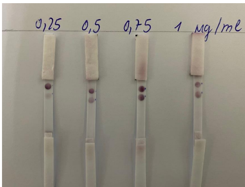
Figure 3. Selection of the antibody concentration on the detection line
