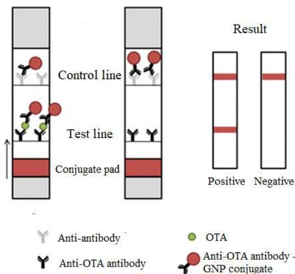
Figure 1. Illustration of the immunochromatographic lateral flow strip test
