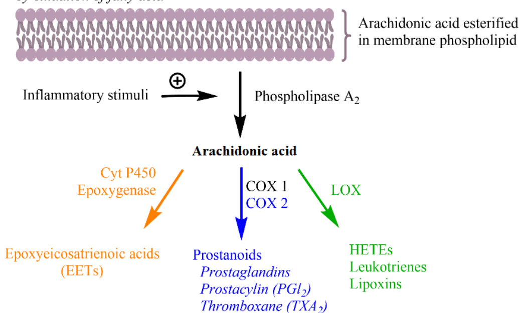
Figure 12. Eicosanoids signaling pathway. Hydroxy Eicosatetraenoic (HETE); Prostaglandin-endoperoxide synthase 1/2 (COX1; COX2).
